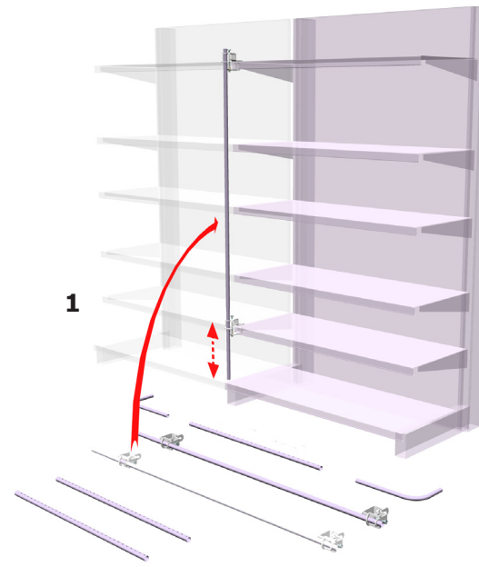
1 mount the pre-assembled side support
