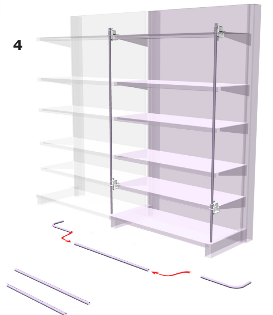
4 assemble the top part
