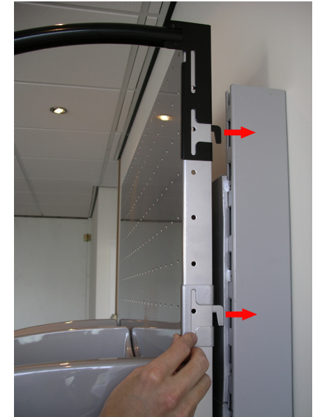
positioneer beiden haken
