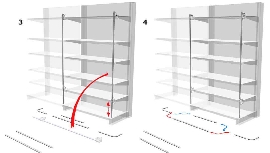
3 mount the 2nd pre assembled side support and adjust to height
