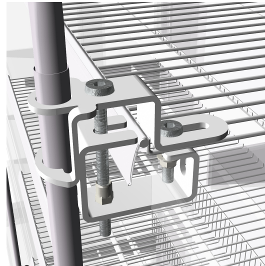
typical wire shelf situation note the additional bolt on shelf
