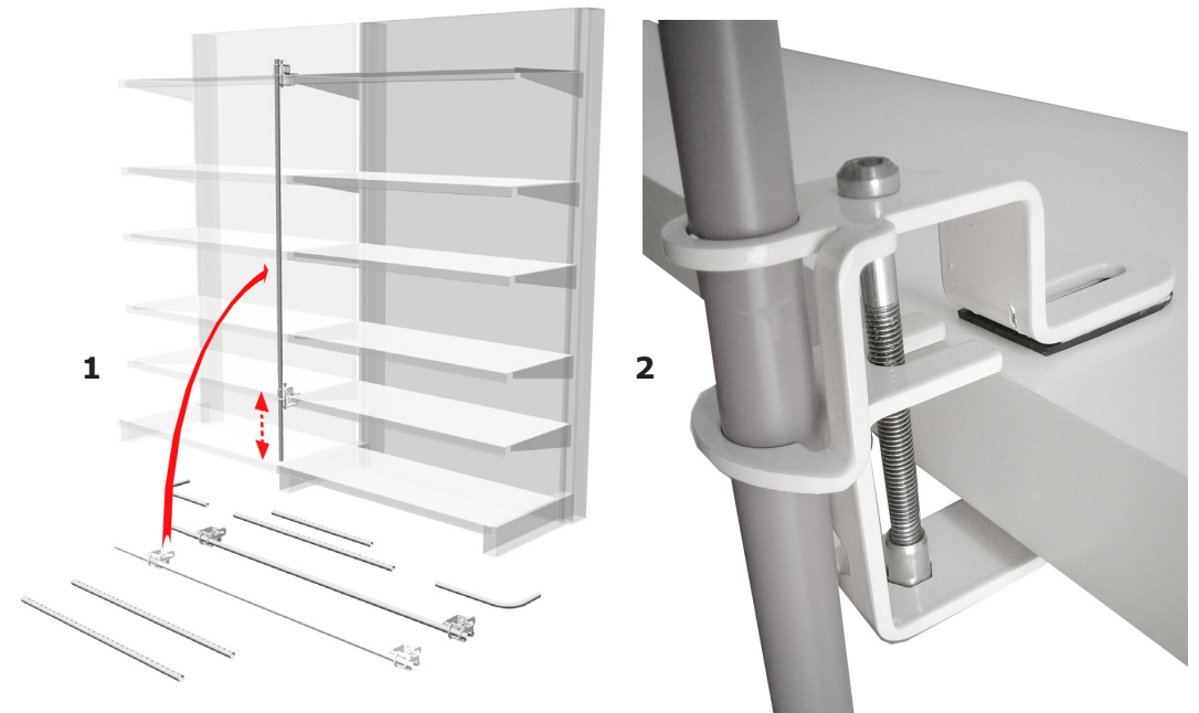
1 mount the pre-assembled side support
