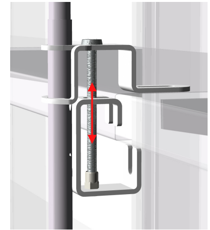
sliding part vertical used with limited back space
