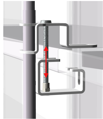
sliding part in general position will suit standard shelves
